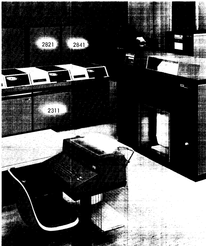
Figure 19. IBM 2311 Disk Storage Drive, 2841 Storage Control Unit, and 2821 Control Unit
