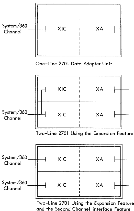
Figure 27. Use of the Expansion Feature and the Second Channel Interface Feature
